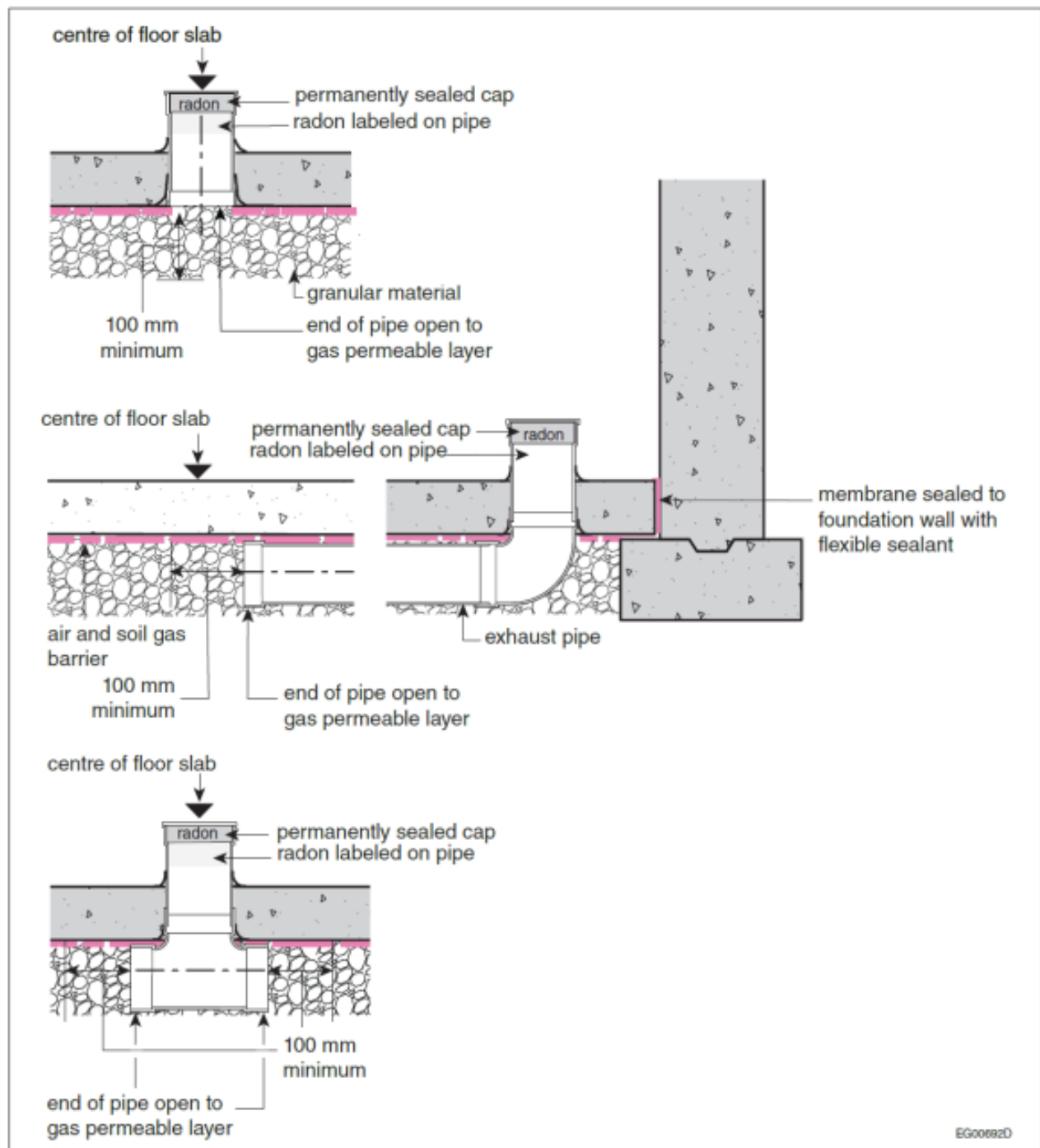
Figure 3 Note 150mm deep granular material required for a radius of 300mm at the centre of slab. Additionally as an alternative to the use of the polyethylene a 75mm 25MPa concrete slab without poly may be used.
