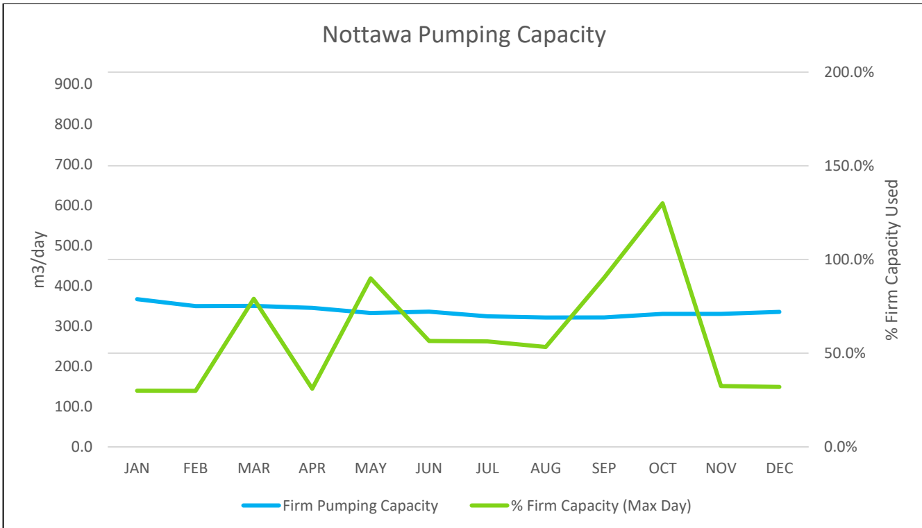
Figure 2: System Capacity
