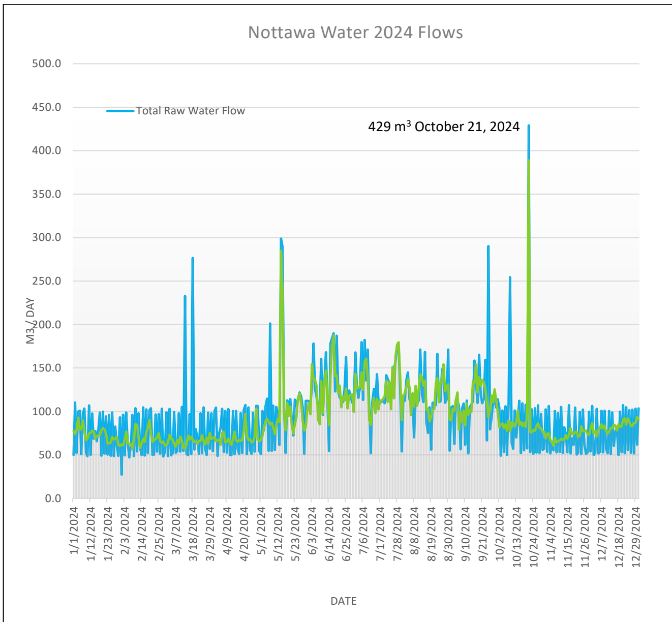
Figure 3: 2024 Daily Flows
