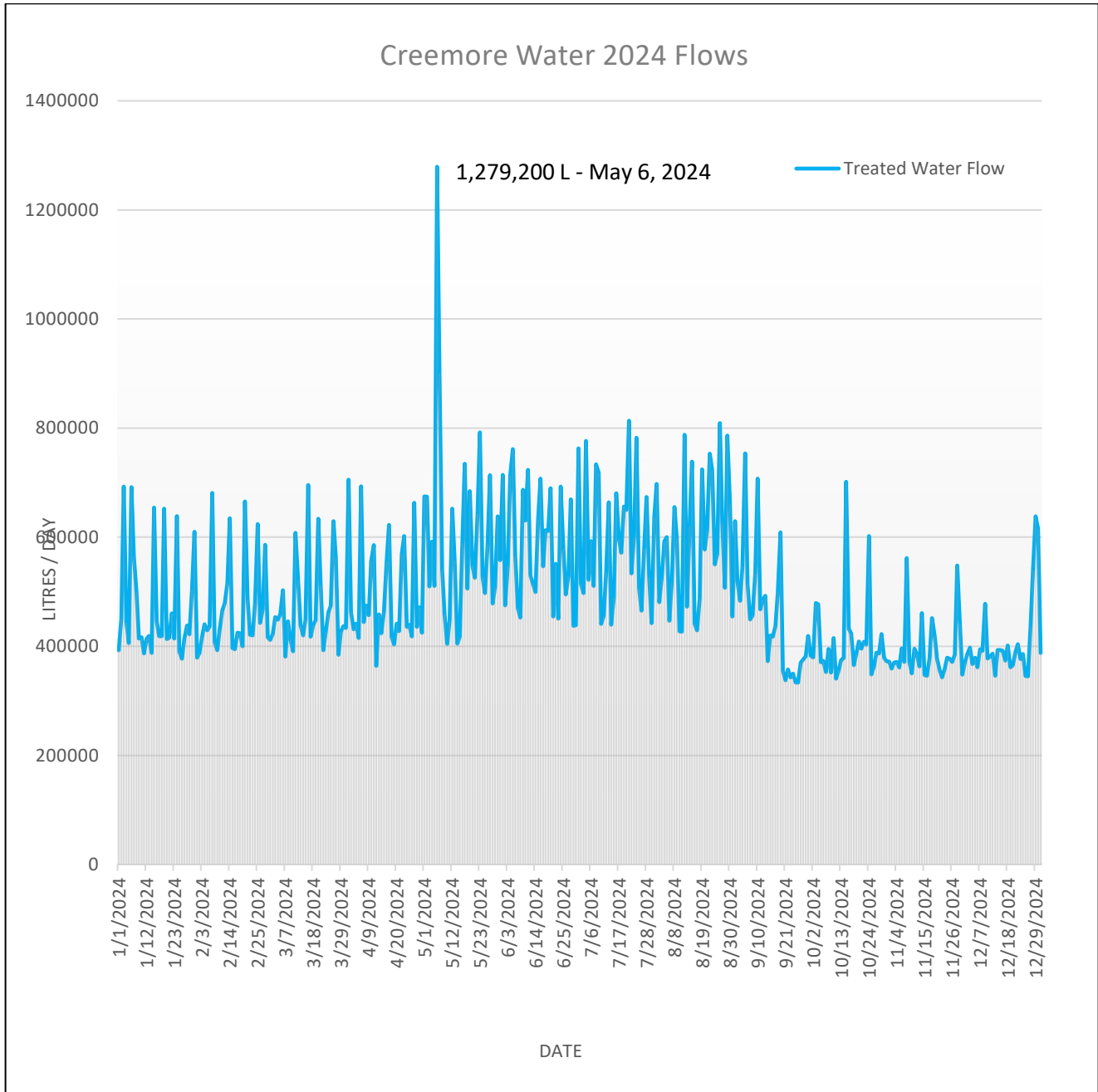
Figure 3: 2024 Daily Flows
