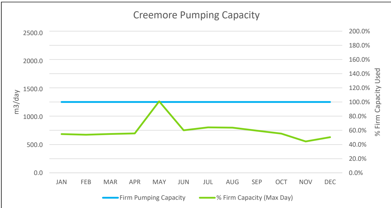
Figure 2: System Capacity
